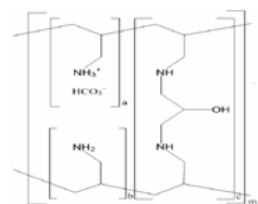
Figure 1. Chemical structure of Sevelamer Carbonate
